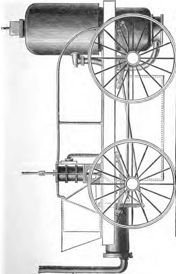
Fig. 17.—The "Novelty," 1825.
